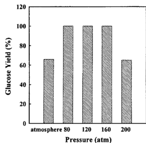
Fig. 4. Effect of pressure on Avicel hydrolysis under supercritical carbon dioxide at 50 °C for 90 min.
